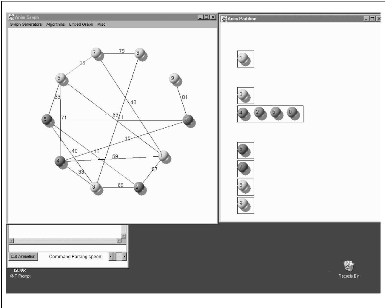
Figure 6: The animation at the fourth step: edges (2,5) , (0,5) and (4,0) have been examined and colored blue together with their endpoints, and the edge (6,7) is currently examined and colored green. The state of the partition is shown to the right: we have grown only one blue tree (containing vertices 0,2,4,5 ). All the other vertices are still in singleton trees.
