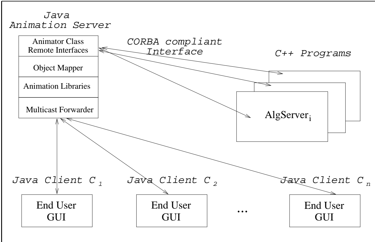
Figure 2: CATAI Basic Architecture.
