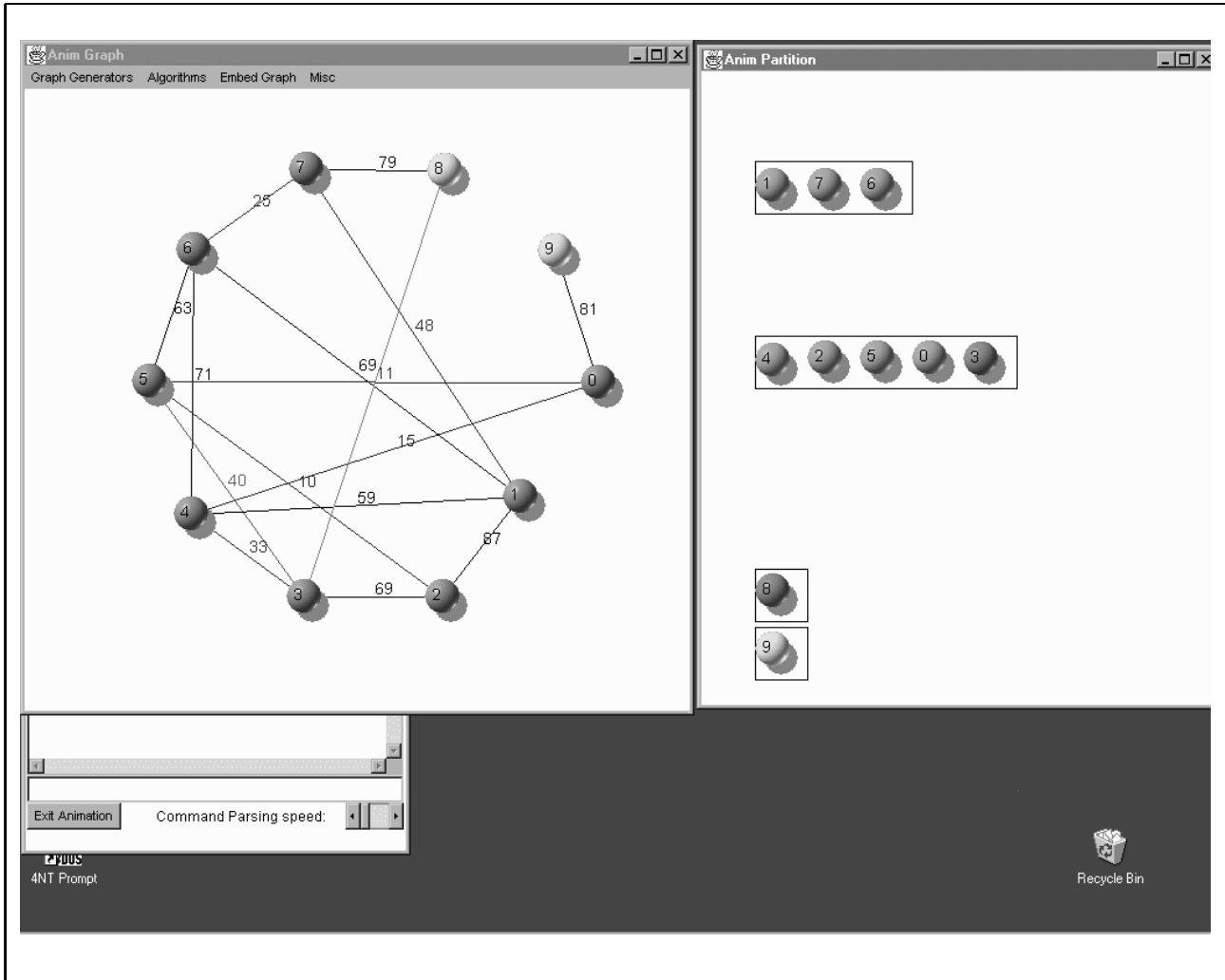
Figure 7: The animation at the eighth step: edges (2,5) (0,5) , (4,0) , (6,7) , (4,3) and (1,7) have been examined and colored blue together with their endpoints, edge (5,3) has been colored red, and the edge (3,8) is currently examined and colored green. The state of the partition is shown to the right: we have grown two blue trees (one containing vertices 0, 2, 3, 4, 5 and the other containing vertices 1, 6, 7 ). Vertices 8 and 9 are still in singleton trees.
