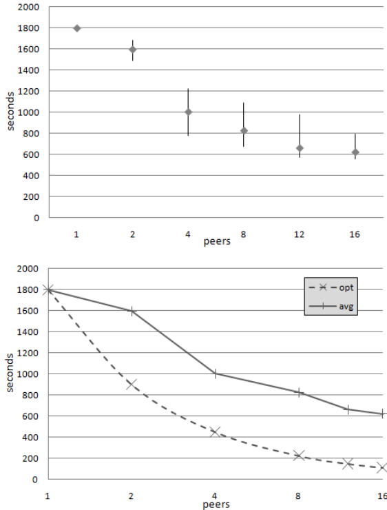
Figure 2. Simulation duration: (top) average and boundaries (bottom) compared with the optimal linear speedup.
